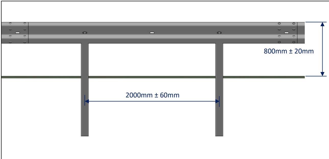
Figure 18: Recommended Installation Tolerances.
