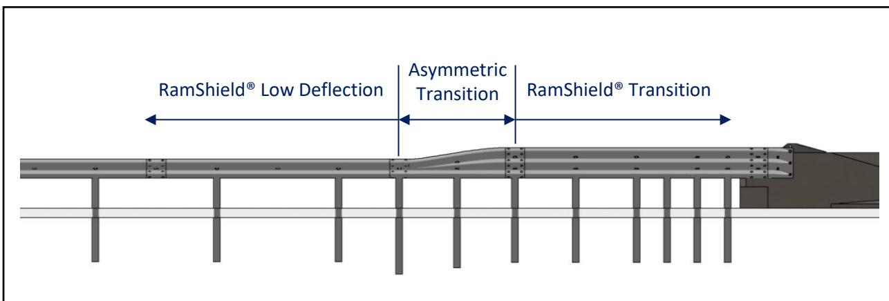
Figure 7: RamShield® Low Deflection, Connection to the RamShield® Transition.
