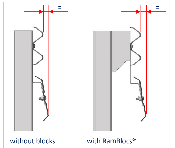
Figure 10: Vertical Alignment of BikerShield™
