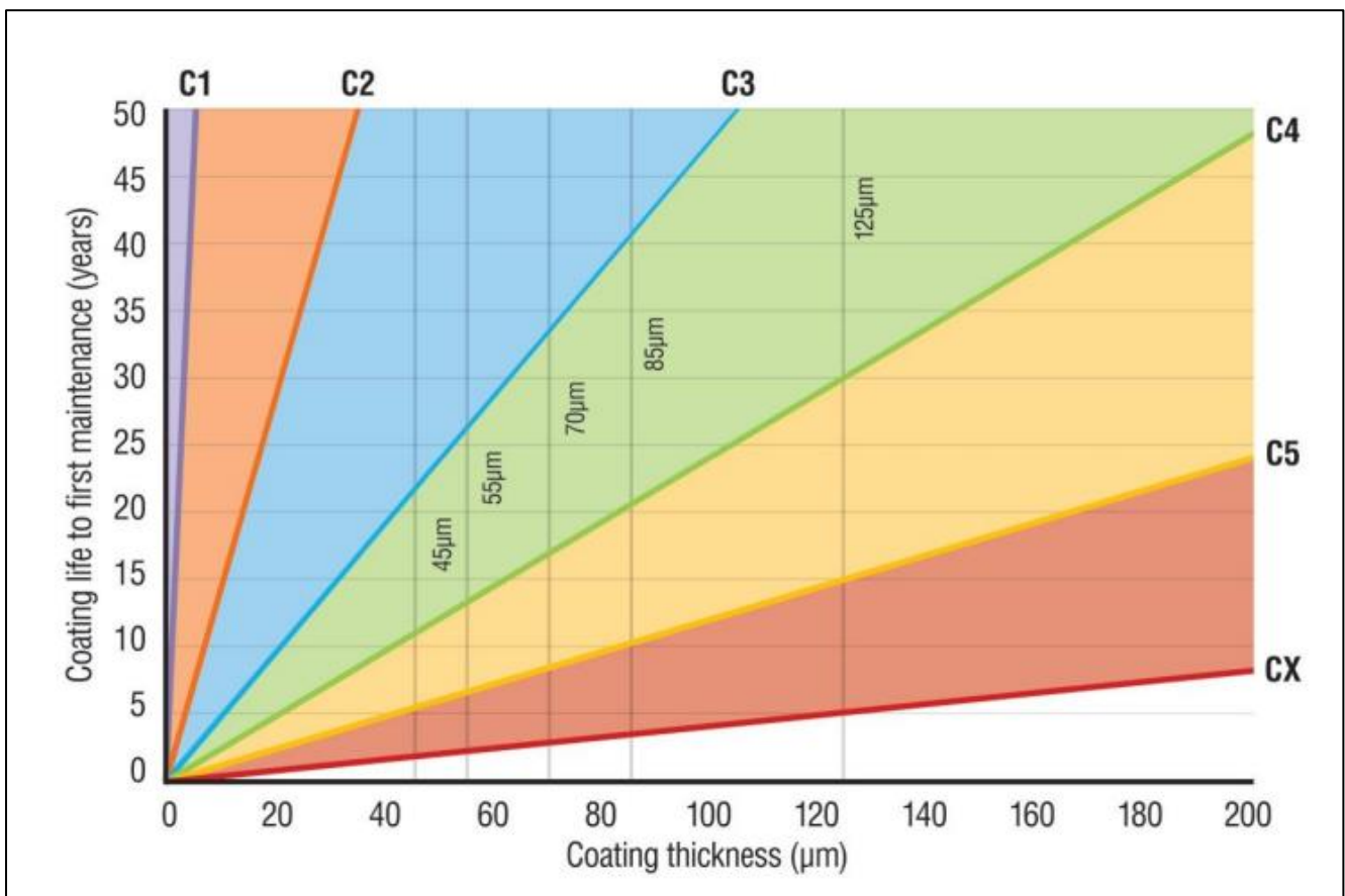
Figure 17: Calculated Corrosivity Rates for Hot Dip Galvanised Coatings from AS/NZS 2312.2
