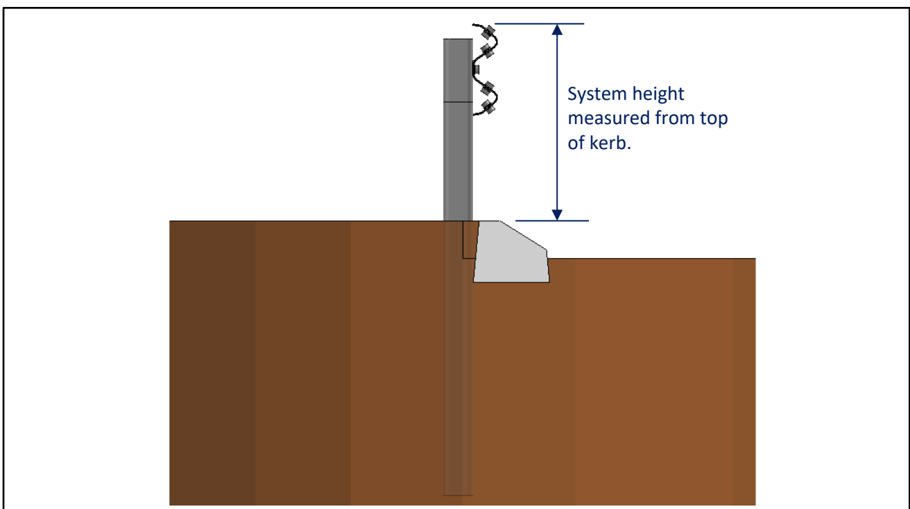
Figure 4: RamShield® Installation Behind a Mountable Kerb.
