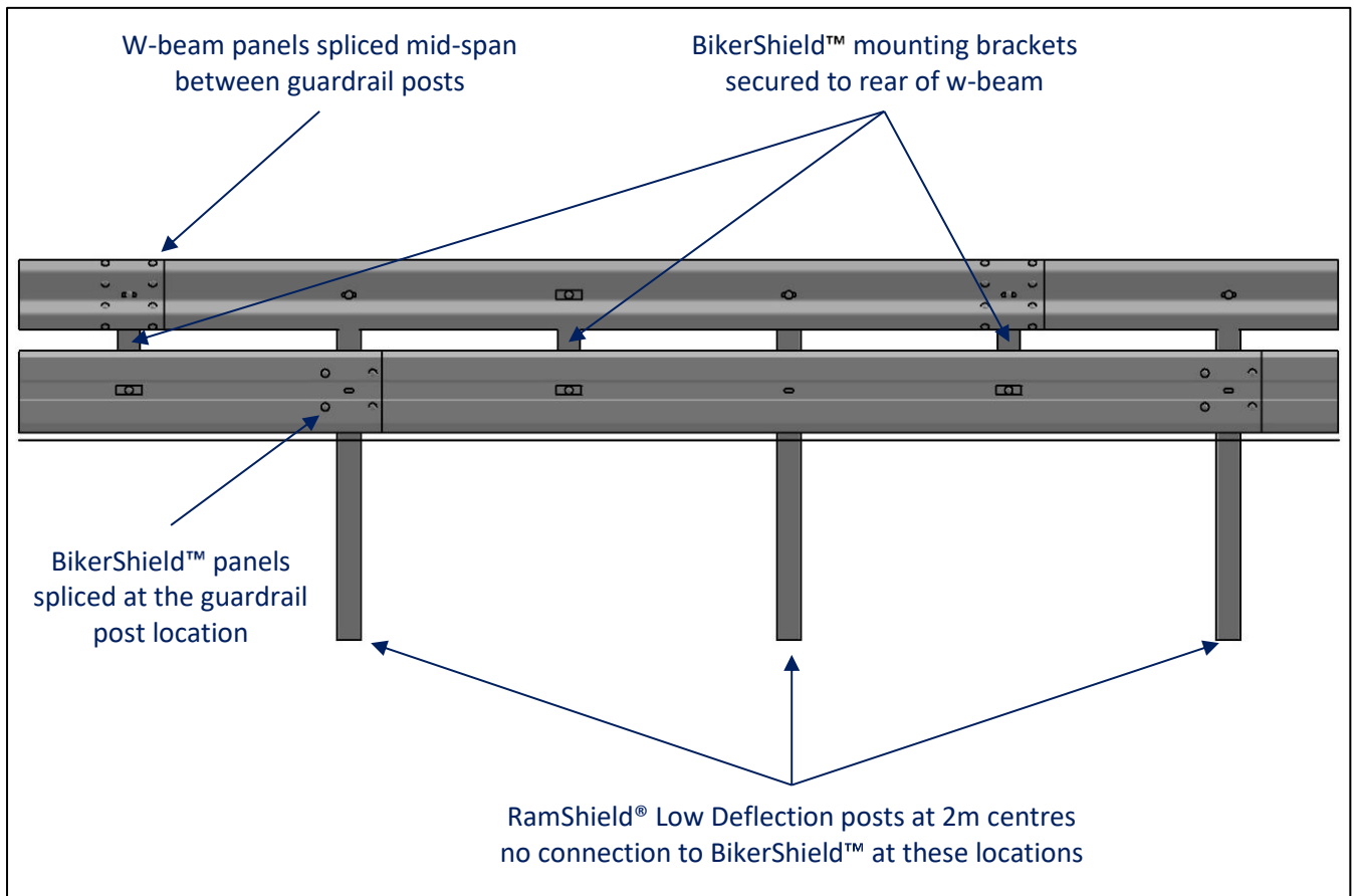
Figure 11: Attachment of BikerShield™ to RamShield® Low Deflection - Front View
