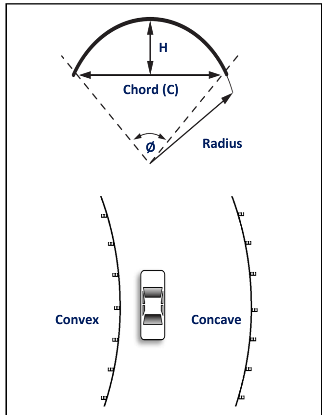
Figure 16: Horizontal Curving of W-Beam Guardrails
