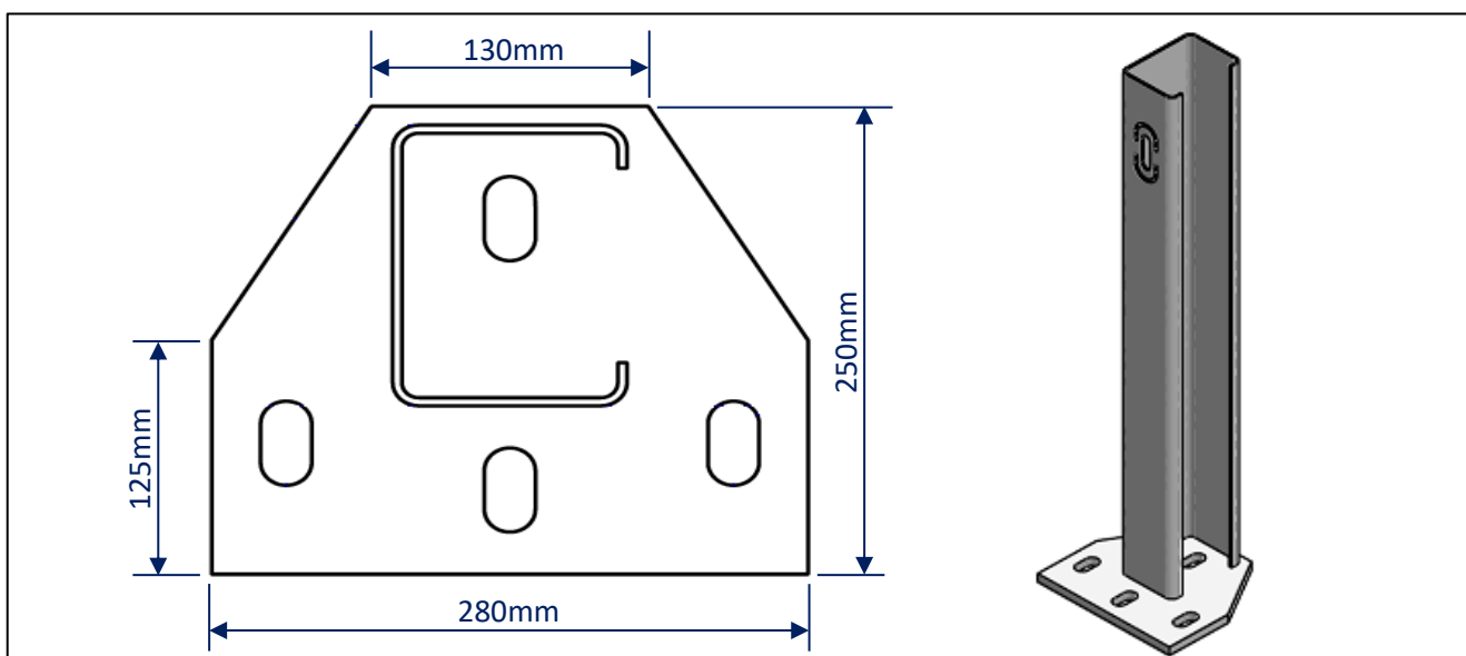
Figure 14: RamShield® Low Deflection Post on Baseplate
