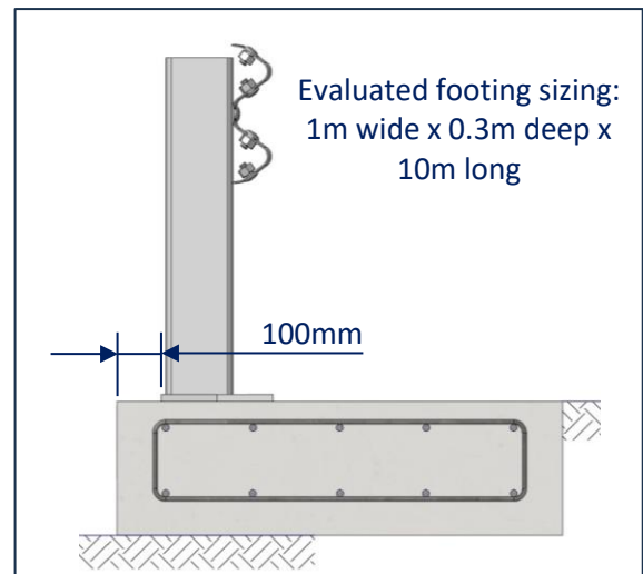
Figure 12: Post Evaluated at Rear of Footing
