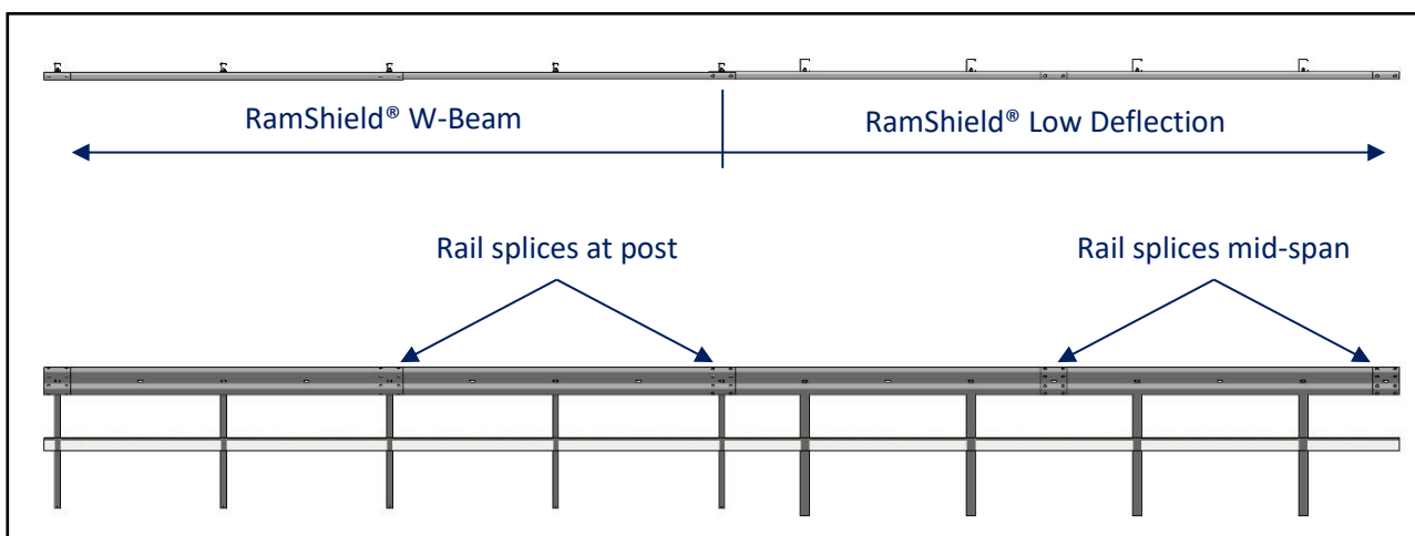
Figure 9: RamShield® Low Deflection, Connection to RamShield® W-Beam.
