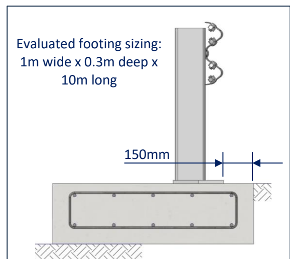
Figure 13: Post Evaluated at Front of Footing
