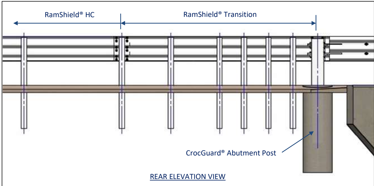
Figure 6: CrocGuard® Connection to RamShield® HC
