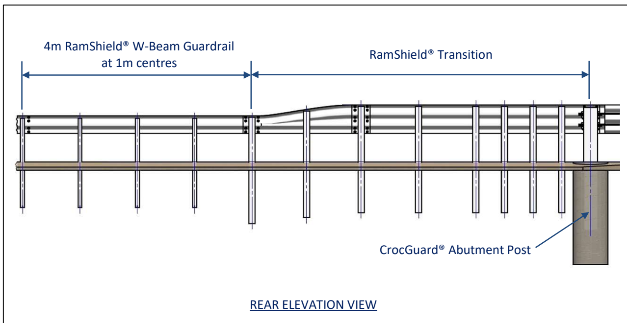
Figure 5: CrocGuard® Connection to RamShield® W-Beam
