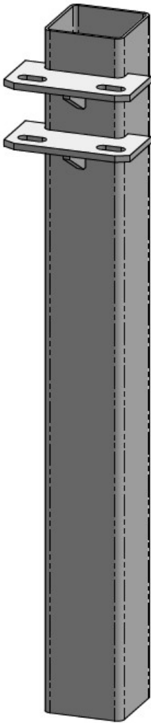
2150mm Abutment Post 250x250x9 SHS 150 kg each
