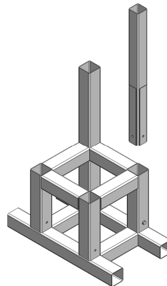
Installation Support Frame 16 kg each (SWL 5 tonnes)
