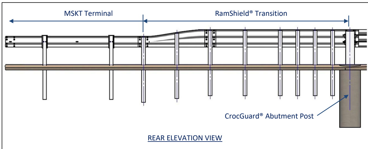
Figure 7: CrocGuard® Connection to MSKT Terminal
